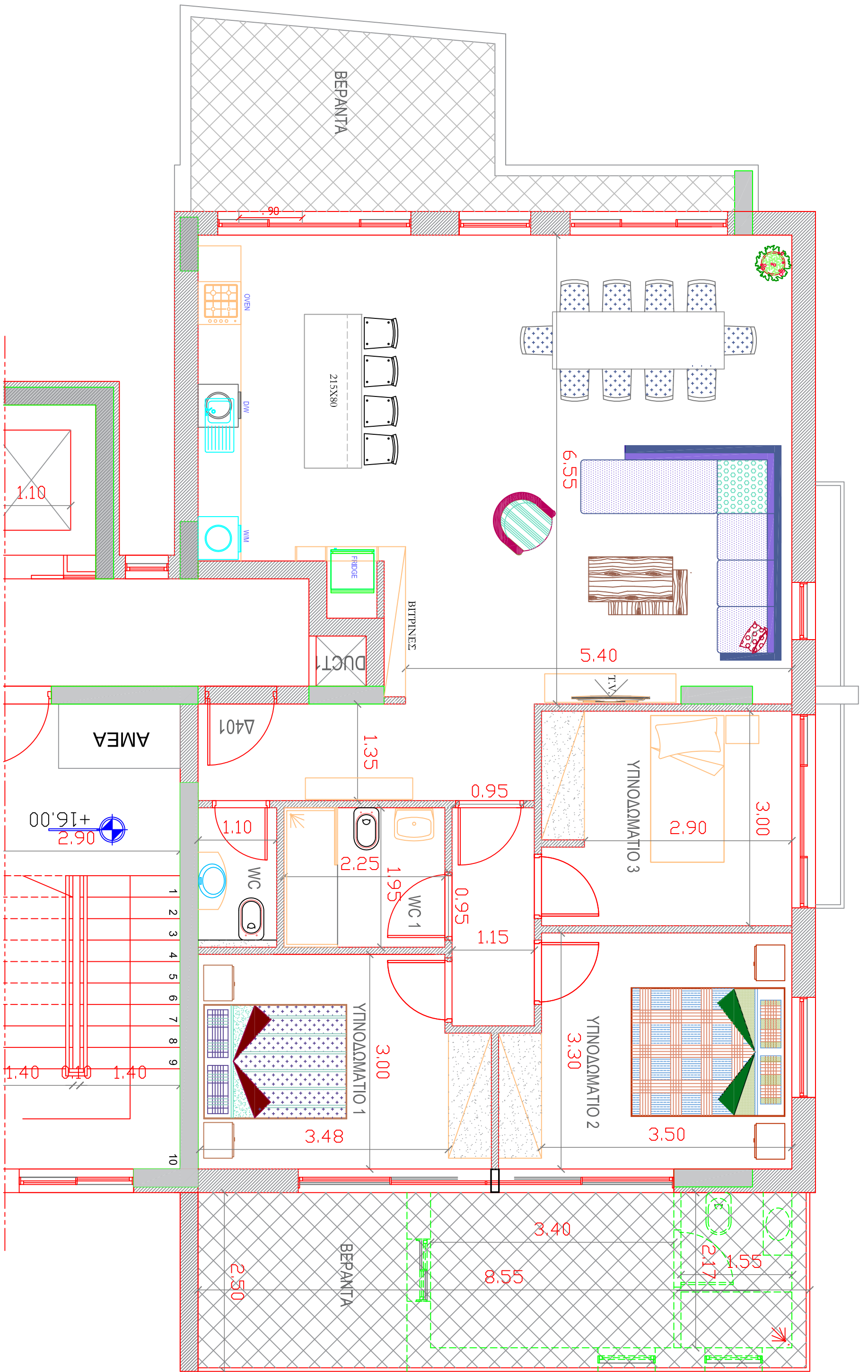
1 1:50 ENDLESS VIEW - FLAT 401 FURNITURE PLAN
